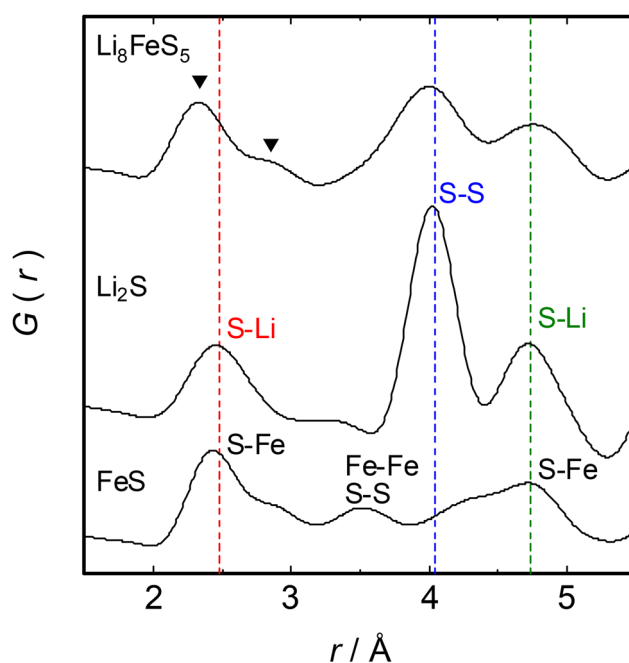
Fig. 2 X-ray RPDF data of \text{Li}_8\text{FeS}_5 . Data for \text{Li}_2\text{S} and \text{FeS} are also shown for comparison.
