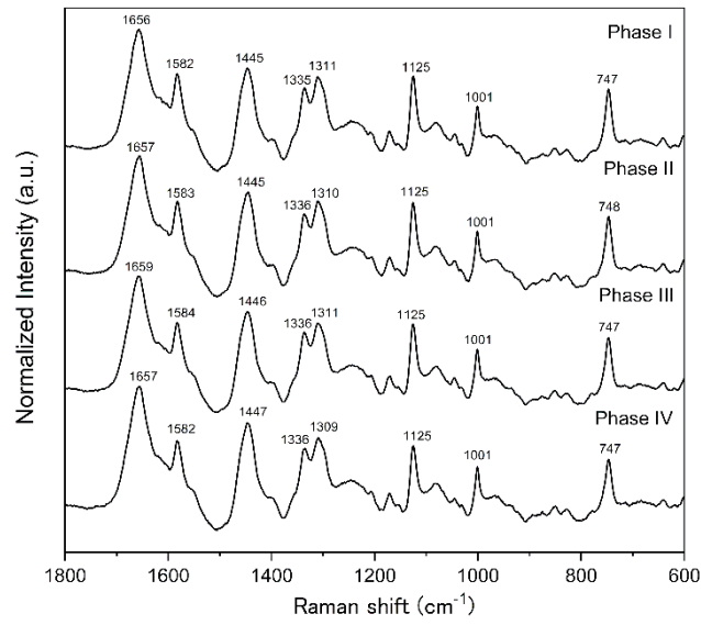
Figure 2: Averaged Raman spectra in 1800–600 \text{cm}^{-1} region for mouse oocytes obtained at Phases I (n=44), II (n=58), III (n=59), and IV (n=57).
