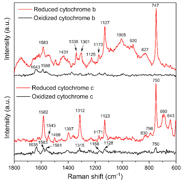
Figure 3: (A) UV-Vis absorbance spectra (460-600 nm) and (B) 532-nm-excited Raman spectra ( 1800\text{-}600\text{ cm}^{-1} ) of oxidized and reduced cytochrome b and c .
