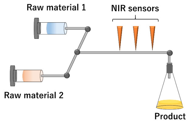
Figure 1: Schematic of a microflow reactor.
