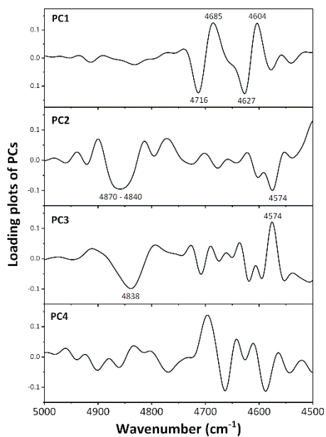
Figure 5: Score plots of (A) PC1 vs. PC2 and (B) PC3 vs. PC4. (C) Loading plots of PC1, PC2, PC3, and PC4.
