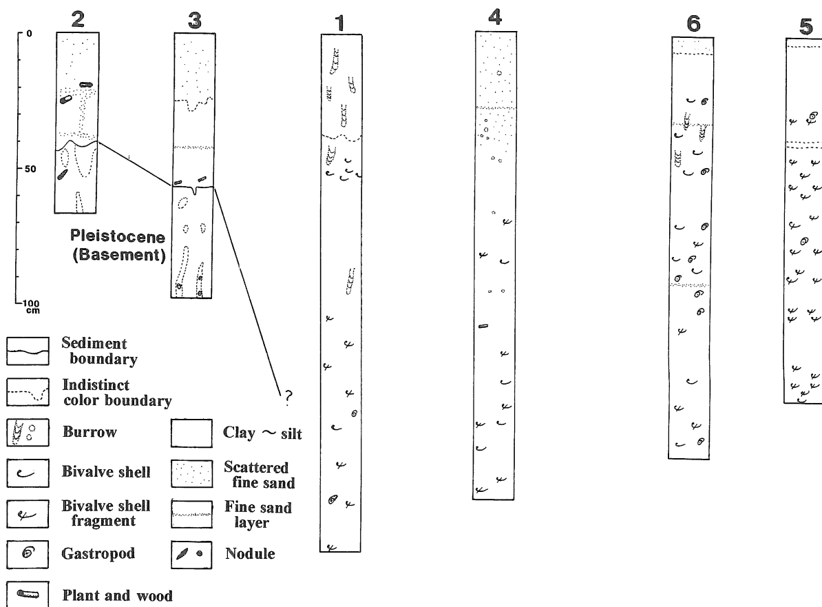
Fig. 2 Columnar sections of the sediments in Lake Cootharaba and Lake Cooroibah
