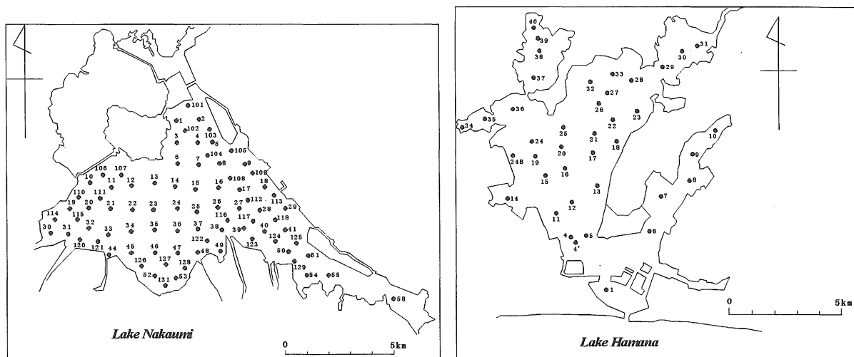
図2. 試料採取地点；(a) 中海, (b) 浜名湖 Fig.2 Sampling stations in Lake Nakaumi (a) and Lake Hamana (b)
