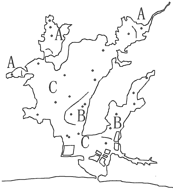
図 3. 浜名湖における群集区分 Fig.3. Distribution of ostracod biofacies in Lake Hamana.
